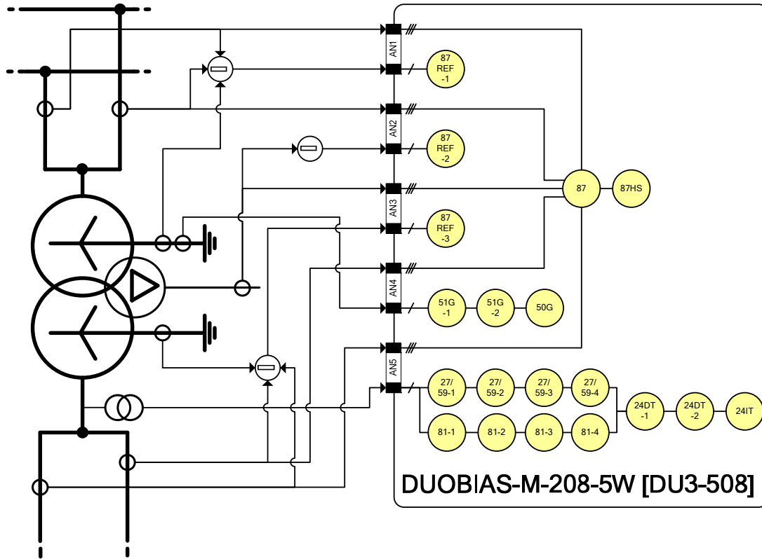
Figure 1 - Duobias-M-208-5W [DU3-508]
